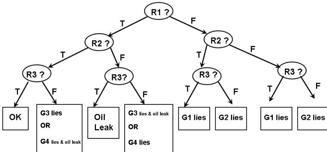
Figure2. The Decision Tree for the Pipeline Example
