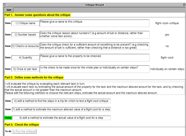
Figure 4: A screenshot from the PSMTTool interface.
