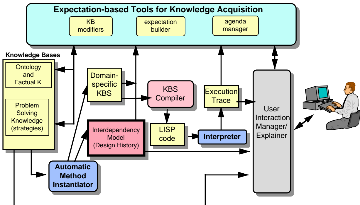
Figure 1: EXPECT Architecture
