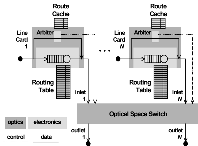
Fig. 2. The Architecture of the Optically Boosted Router
