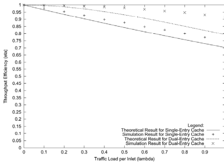
Fig. 4. Comparison of Theoretical and Simulation Results for a Booster with 3 Links.
