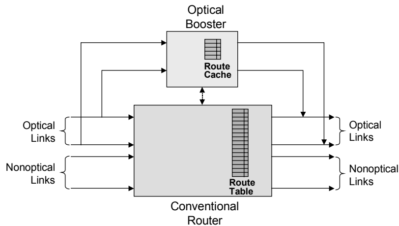
Fig. 1. A Base Router Enhanced by a Boosting Router
