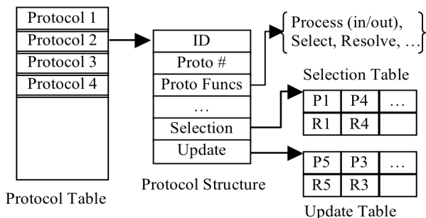
Figure 1. Flexible Stack Architecture
