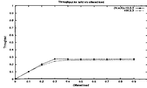
Fig. 4. Throughput for the Is/Id mechanism ( Th_{isid} ) against offered load. The average packet length was 500 bytes and the chipping rate was 1Gb/s. The thresholds used were thresh_m = 2 for both codesets and thresh_c = 4 for the (10, 3, 3) codeset and thresh_c = 40 for the (100, 3, 3) codeset
