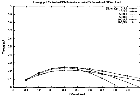
Fig. 3. Network throughput ( T_{\text{aloha-cdma}} ) against offered load for different codeset design parameters ( N, w, \kappa ) for Aloha-CDMA from analysis. The average packet length was 500 bytes and the chipping rate was 1Gb/s.
