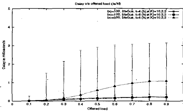
Fig. 6. Delay against offered load using realistic network traces for the Is/I_d mechanism. Plots are shown for different values of the backoff timer( bt ), backoff count( bc ) and overlap threshold( t ).
