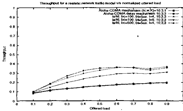
Fig. 5. Throughput against offered load using realistic network traces for the Aloha-CDMA mechanism and Is/I_d . Plots are shown for different codesets (for Aloha-CDMA) and different values of the backoff timer( bt ), backoff count( bc ) and overlap threshold( t ) (for Is/I_d ).
