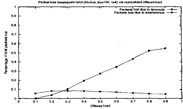
Fig. 7. Breakdown of the fraction of packets dropped (as a fraction of the total packets sent) against offered load using realistic network traces for the Is/I_d mechanism and a (10, 3, 3) code.
