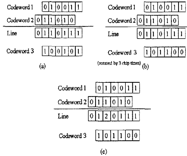
Fig. 1. Examples of interference between codewords
