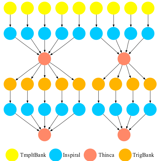
Figure 5. LIGO workflow
