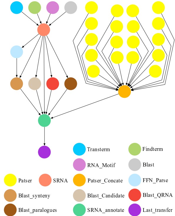
Figure 6. SIPHT workflow
