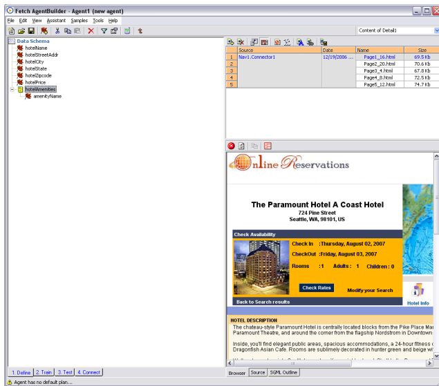
Figure 1: Schema definition for a hotel agent using the “OnlineReservations” site. The user defines output fields such as “hotel name” and “hotel city”, then drags the relevant text from the page over each output field for each page used in training.
