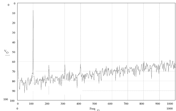
Figure 11: The modulator output spectrum with a 100 KHz sinusoid input.
