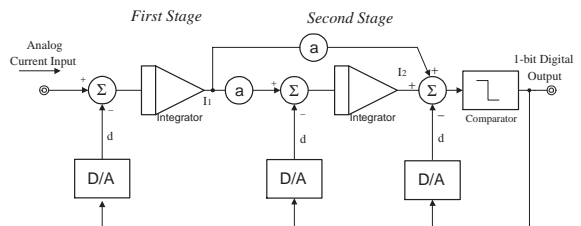
Figure 4: The block diagram of a second-order \Sigma\Delta modulator with reduced delay.
