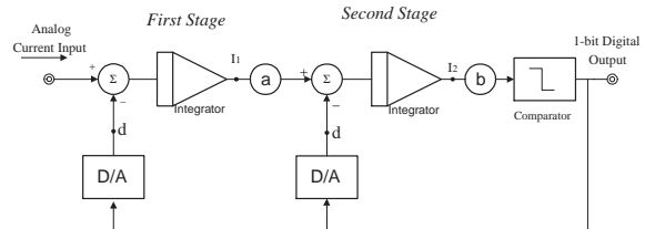
Figure 3: The block diagram of a second-order \Sigma\Delta modulator.
