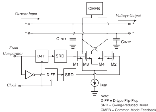
Figure 2: The simplified scheme of the high-speed current switch.
