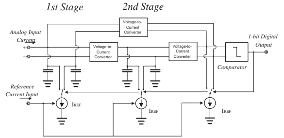
Figure 6: The architecture of the new second-order continuous-time switched-current \Sigma\Delta modulator.
