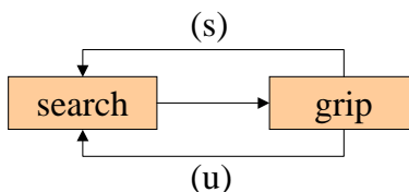
Figure 6: Macroscopic state diagram of the multi-robot system. The arrow marked ‘s’ corresponds to the transition from the gripping to the searching state after a successful collaboration, while the arrow marked ‘u’ corresponds to the transition after an unsuccessful collaboration, i.e. , when the robots time out.
