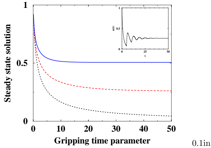
Figure 7: Steady state solution vs (dimensionless) gripping time parameter \tau : for \beta = 0.5 (short dash), 1 (long dash), 1.5 (solid line). Inset shows a typical relaxation to the steady state for \tau = 5 , \beta = 0.5 .
