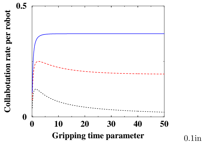
Figure 8: Collaboration rate per robot vs (dimensionless) gripping time parameter \tau for \beta = 0.5 (short dash), \beta = 1 (long dash), \beta = 1.5 (solid line). These values of \beta correspond, respectively, to two, four, and six robots in the experiments with four sticks ( cf. Fig. 5).
