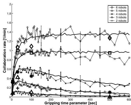
Figure 5: Collaboration rate as a function of the gripping time in homogeneous groups of two to six robots and four sticks. The large single markers correspond to the results with the real robots, the linked small markers to those with the Webots simulator, and the underlying continuous lines to those with the probabilistic simulation (from Ijspeert et al. [14]).
