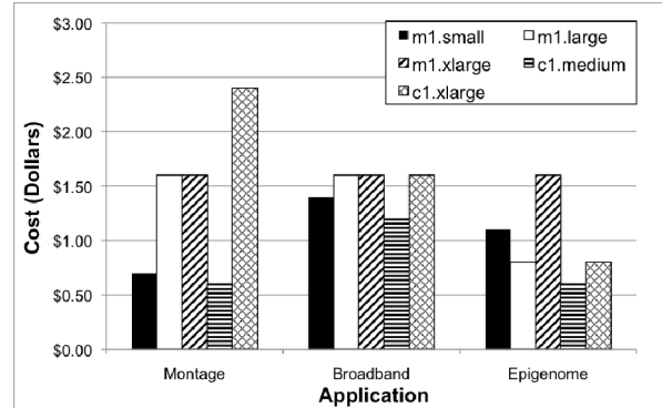
Figure 2. The processing costs for the Montage, Broadband and Epigenome workflows for the Amazon EC2 processors given in the legend.
