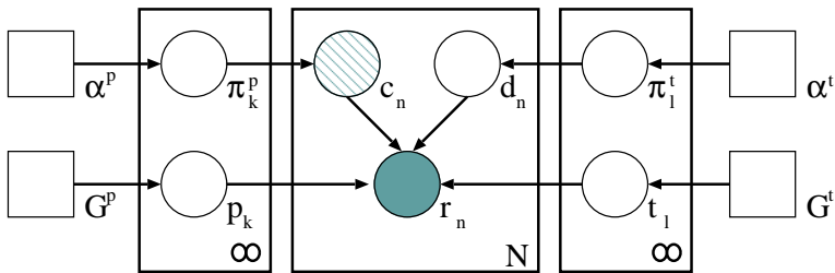
Figure 1: Graphical model for our generic supervised clustering model.
