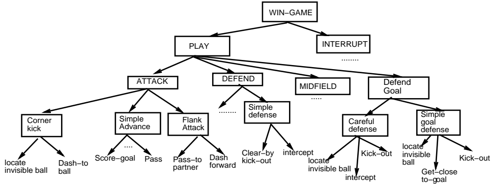
Figure 1: A portion of the operator hierarchy for player-agents in RoboCup soccer simulation. Boxed operators are team operators, others are individual operators.
