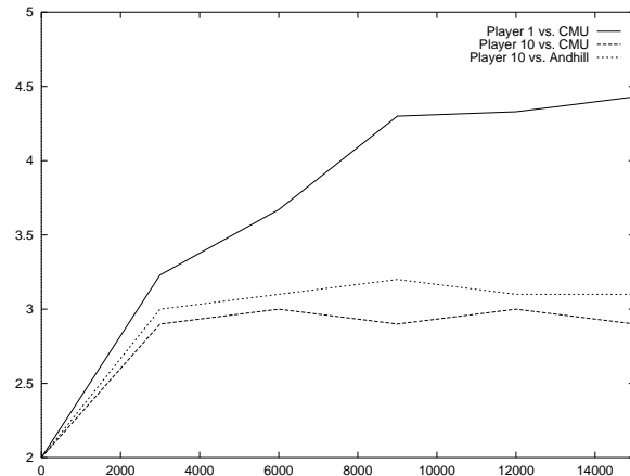
Figure 3: Contrast of Player 1 versus CMUnited with Player 10 versus both CMUnited and Andhill, under the same input condition. Player 1 is a forward and Player 10 is a goal defender.
