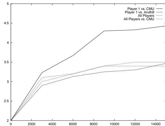
Figure 2: Contrast of Player 1 versus CMUnited with Player 1 versus Andhill under same input condition. Means across all players provided for comparison. Player 1 is a forward.
