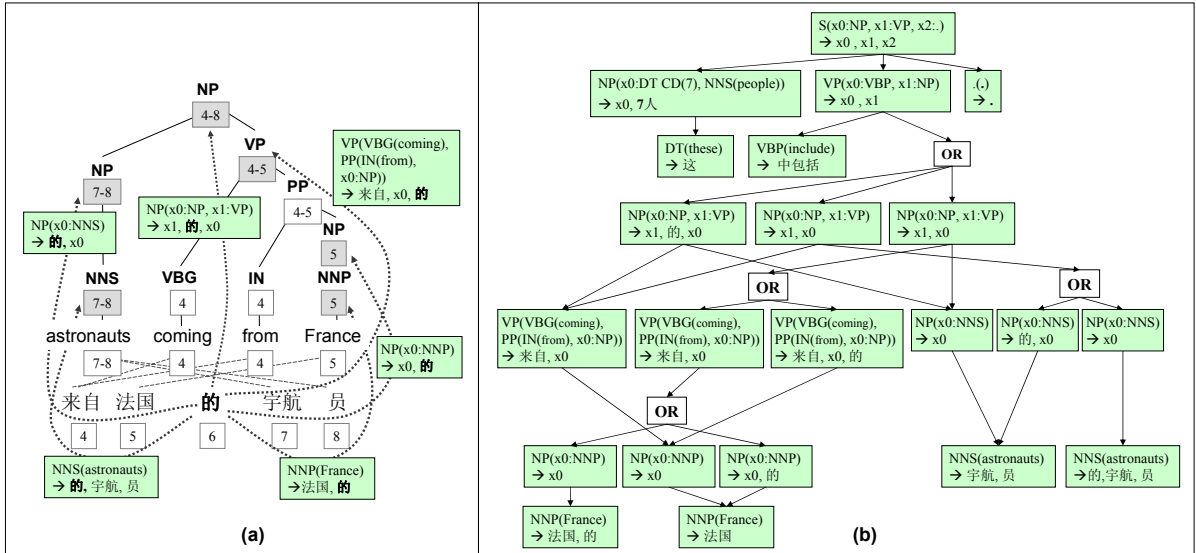
Figure 2: (a) Multiple ways of aligning 的 to constituents in the tree. (b) Derivation corresponding to the parse tree in Figure 1, which takes into account all alignments of 的 pictured in (a).
