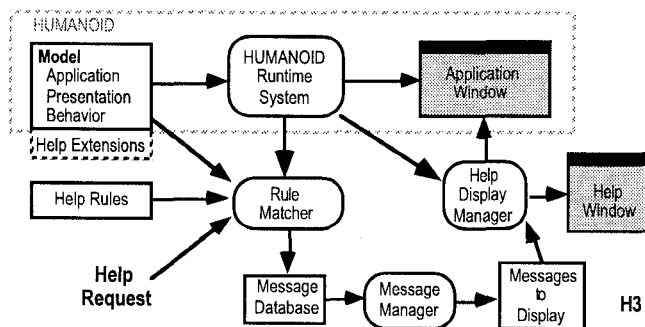
Figure 4. Architecture of H3. HUMANOID provides the enabling technology that allows H3 to access the information it need to construct the help messages and highlight the appropriate portions of the display.
