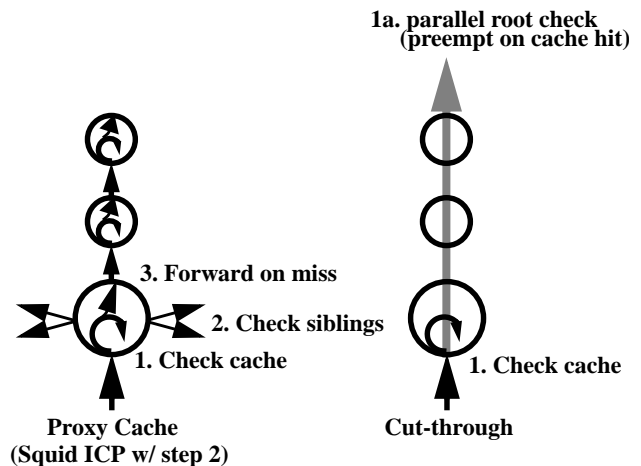
FIGURE 8. Check-and-forward vs. cut-through (black is foreground, grey is background)
