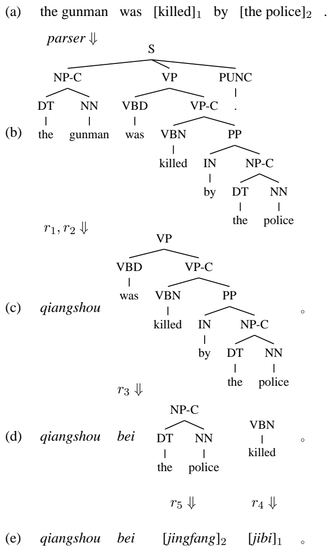
Figure 2: A syntax-directed translation process for Example (1).
