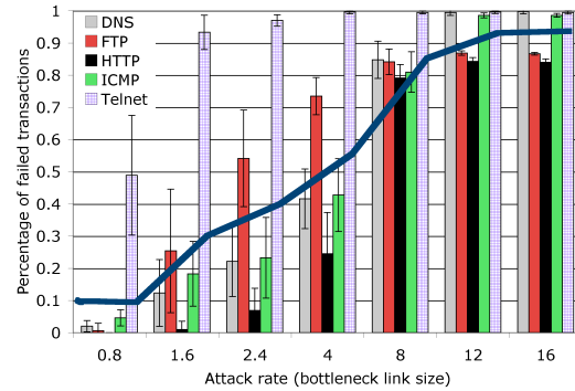
(b) DoS-hist measure vs attack strength
