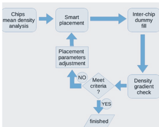
Figure 1. MPW chip placement flow optimizing density and density gradients between chips on the MPW reticle.
