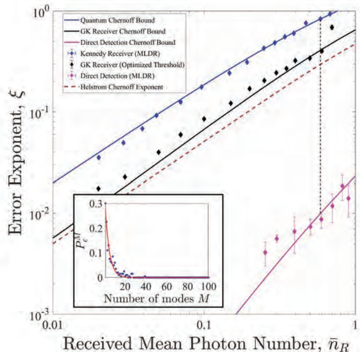
Data shows experimental validation of the measurement to achieve the quantum Chernoff bound
