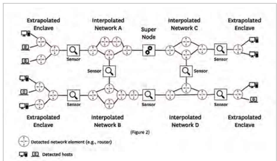
Inferred topology based on measurements from sensors
