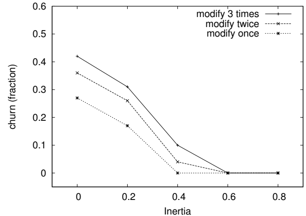
Figure 5: Effects of different inertia on representative churn (HL28/16 modified three times by it29w through it31w; modified twice by it29w, it30w; and once by only it29w).
