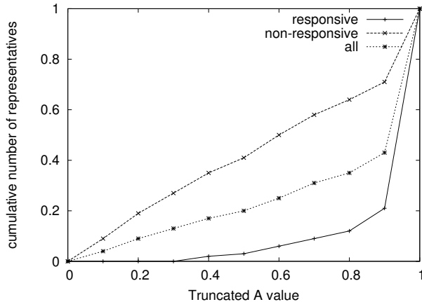
Figure 3: A^t cumulative distribution on responsive part of N_p , non-responsive part of N_p and all N_p
