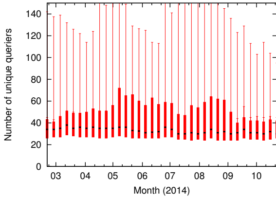
Figure 8: Box plot of originator footprint (quiers per scanner) over time; whiskers: 10%ile/90%ile. (Dataset: M-sampled.)
