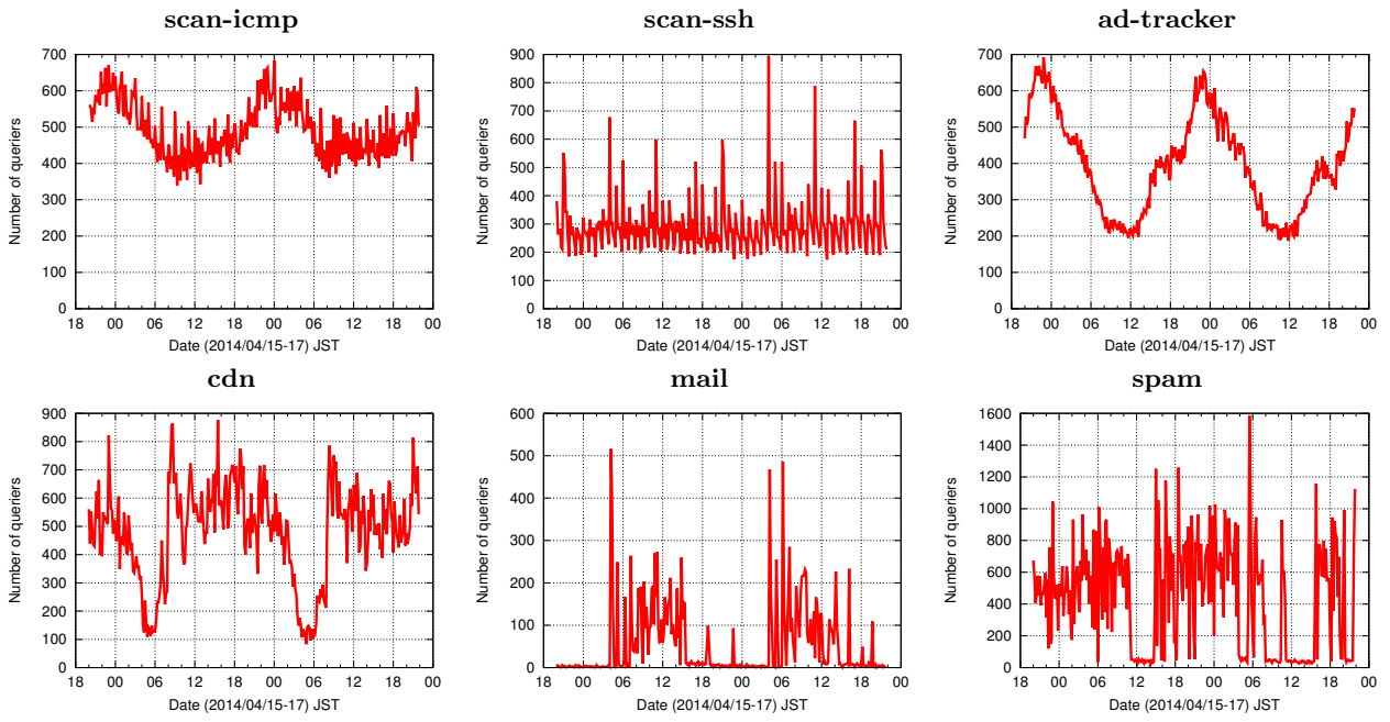
Figure 12: Counts of queries per minute over 50 hours for Daily variation in number of queriers for our case studies. (Dataset: JP-ditl.)
