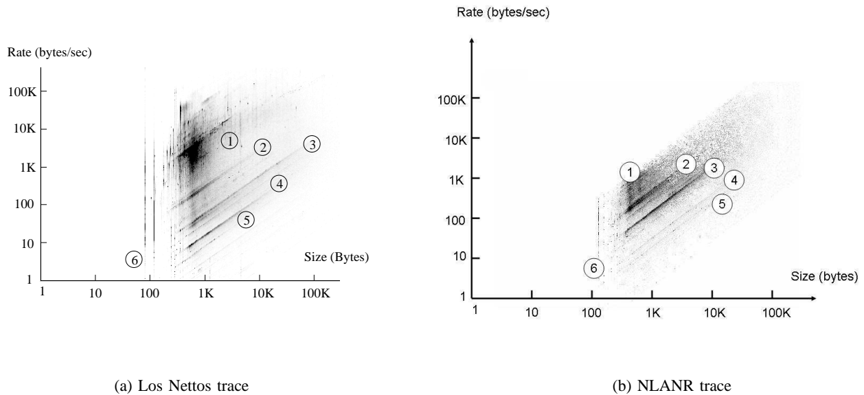
Fig. 3. Density plots of size and rate for TCP flows (at log-log scale)
