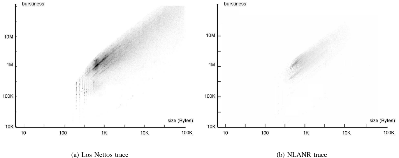
Fig. 10. Density plots of size and burstiness for TCP flows
