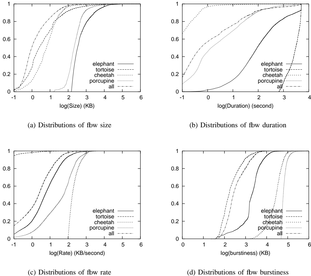
Fig. 1. The relationship between different characterizations of heavy-hitter flows
