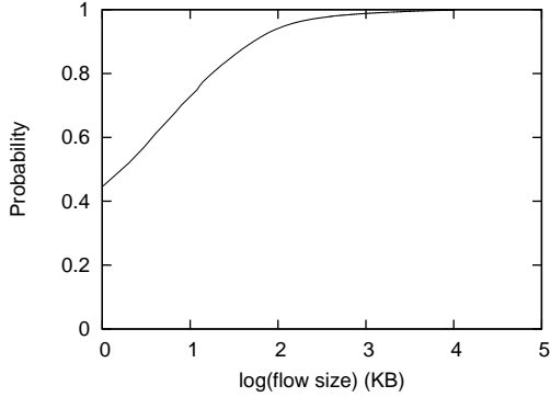
Fig. 2. Distribution of flow size for flows with a duration longer than 30 seconds in Los Nettos trace
