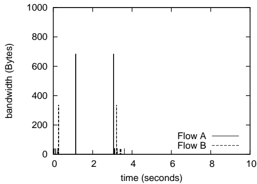
Fig. 13. Bandwidth-time plots of flow A and B
