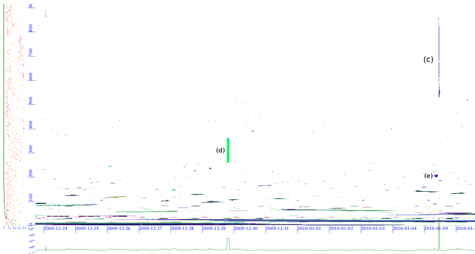
Fig. 2: The 900 largest outages of Survey S_{30w} , x axis: time, y axis: address space (blocks). Colors represent countries. Subgraphs on X and Y axis show marginal distributions (green line) and overall block responsiveness (red dots). Full interactive graph available as Supplement 5 in [22].
