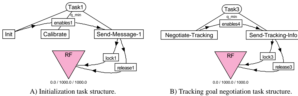
Figure 4: Two TÆMS task structures, abstractions of those used in our agents.
