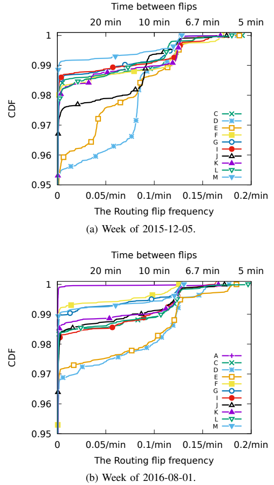
Fig. 2: Cumulative distribution of mean flip time for each VP, broken down by anycast service. (Note the y-axis does not start at zero.)
