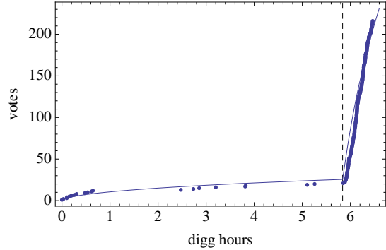
Figure 15: Voting behavior: the number of votes vs. time, measured in Digg hours, for a promoted story in June 2006. The curve shows the corresponding solution from our model and the dashed vertical line indicates when the story was promoted to the front page. This story eventually received 2566 votes.
