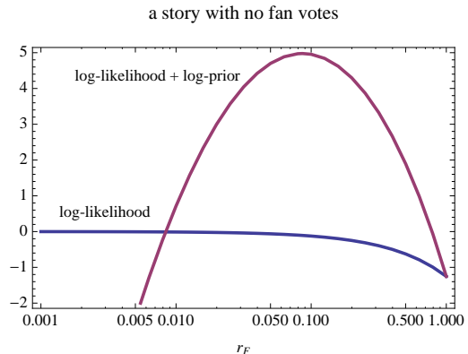
Figure 20: Comparison of log-likelihood (i.e., \log P(r|\text{votes}) ) and log-likelihood plus \log(P_{\text{prior}}(r)) for estimating r_F for a story with no fan votes. The maximum of the log-likelihood is at r_F = 0 while the maximum with the prior is r_F = 0.086 .
