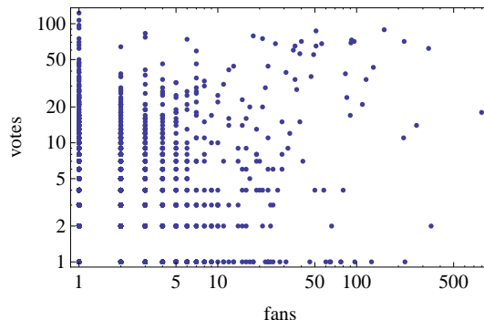
Figure 12: Comparison of activity (number of votes) and number of fans for each of the 3436 users with at least one vote and one fan.
