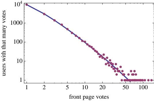
Figure 14: User activity distribution on logarithmic scales. The curve shows the fit to the model described in the text.
