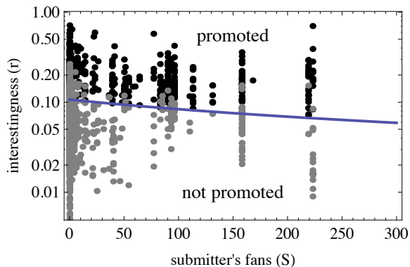
Figure 7: Story promotion as a function of S and r . The r values are shown on a logarithmic scale. The model predicts stories above the curve are promoted to the front page. The points show the S and r values for the stories in our data set: black and gray for stories promoted or not, respectively.
