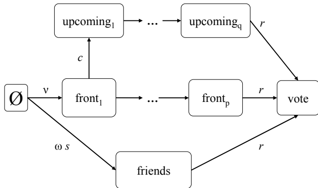
Figure 4: State diagram of user behavior for a single story. A user starts in the \emptyset state at the left, may find the story through one of the three interfaces and may then vote on it. At a given time, the story is located on a particular page of either the upcoming or front page lists, not both. This diagram shows votes for a story on either page p of the front pages or page q of the upcoming pages. Only fans of previous voters can see the story through the friends interface. Users in the friends, front or upcoming states may choose to leave Digg, thereby returning to the \emptyset state (with those transitions not shown in the figure). Users reaching the “vote” state remain there indefinitely and can not vote on the story again. Parameters next to the arrows characterize state transitions.
