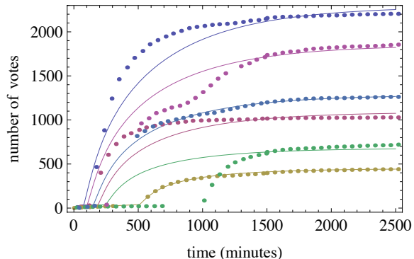
Figure 6: Evolution of the number of votes received by six stories compared with model solution.
