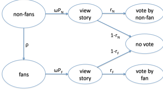
Figure 10: State diagram for a user. The submitter provides a story’s first vote. The initial set of fans consists of the submitter’s fans; other users are initially non-fans. Fans and non-fans have different probabilities to see and vote on the story. With each vote, a non-fan user who is a fan of that voter moves into the fans state. This state transition is caused by the votes of other users: a user moving from the non-fans to fans state is not aware of that change until later visiting Digg and seeing the story in the friends interface.
