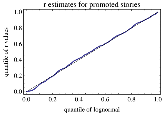
Figure 9: Quantile-quantile plot comparing observed distribution of r values with the lognormal distribution fit (thick curve). For comparison, the thin straight line from 0 to 1 corresponds to a perfect match between the data and the distribution.
