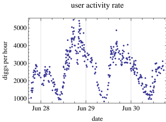
Figure 3: Voting rate (digs per hour) on front page stories at the end of June 2006. The indicated dates are the start of each day (0:00 GMT). The minimum in daily activity is around 9am GMT. Each point is the average voting rate for 100 successive votes.
