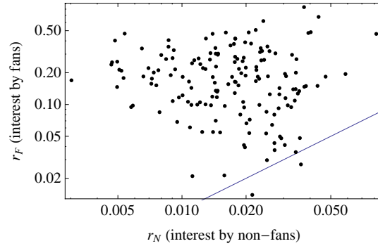
Figure 18: Log-log plot comparing estimated interestingness to fans ( r_F ) and non-fans ( r_N ) for 161 promoted stories with votes from fans (so the estimate of r_F is positive). All the stories in our data set had non-fan votes, giving all the estimates for r_N as positive numbers. The line indicates where r_F = r_N .
