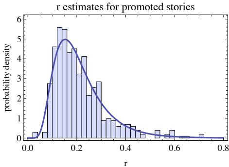
Figure 8: Distribution of interestingness (i.e., r values) for the promoted stories in our data set compared with the best fit lognormal distribution.
