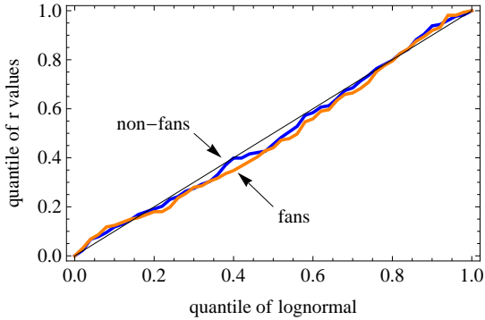
Figure 17: Quantile-quantile plot comparing the observed distribution for r_F (fans) and r_N (non-fans) with the corresponding lognormal distribution fits (thick curves). For comparison, the thin straight line from 0 to 1 corresponds to a perfect match between the data and the distribution.
