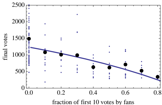
Figure 19: Relation between final number of votes and the fraction of votes by fans among a story’s first 10 votes. Small points are individual stories and the large points are the mean values for each number of votes by fans. The curve shows the model prediction.
