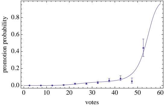
Figure 13: Probability for promotion before the next vote for an upcoming story as a function of the number of votes. The error bars indicate the 95% confidence intervals for the estimates. The curve is a logistic fit.
