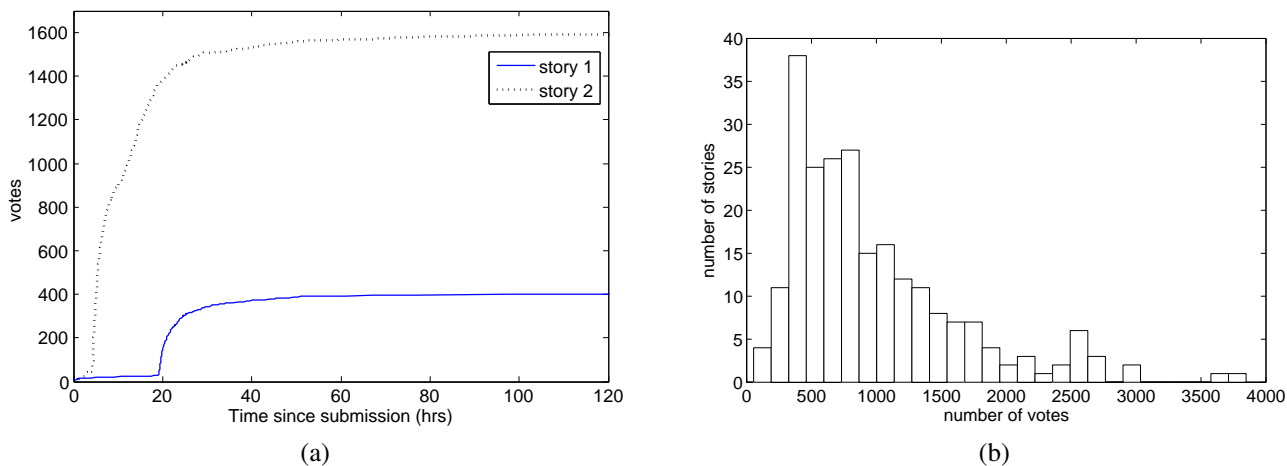
Figure 2: Dynamics of social voting. (a) Evolution of the number of votes received by two front page stories in June 2006. (b) Distribution of popularity of 201 front page stories submitted in June 2006.
