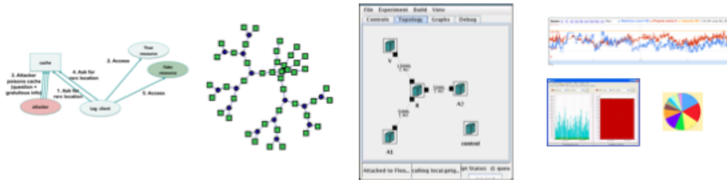
Figure 1: Experiment lifecycle
